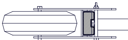
TRANSPORTER SHOWN INSTALLED ON A SOCCER GOAL WITH 4" x 2" UPRIGHTS (No. 467100 GOAL SHOWN)
